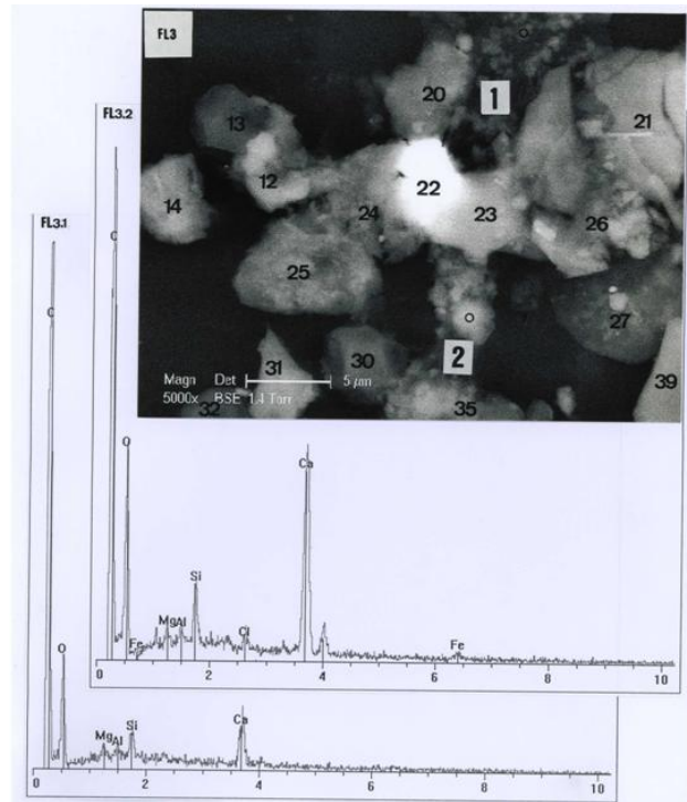
Figure 7. Above, SEM photography (x5000, in BSE). Below, EDX analysis of the first (FL3.1) and the second (FL3.2) parts of FL3 at the white points indicated. FL3 is covered in its middle part by particle b23, and limited at the basis by particle b35. Particles b20, 21 and 22 are adjacent to the fiber.
