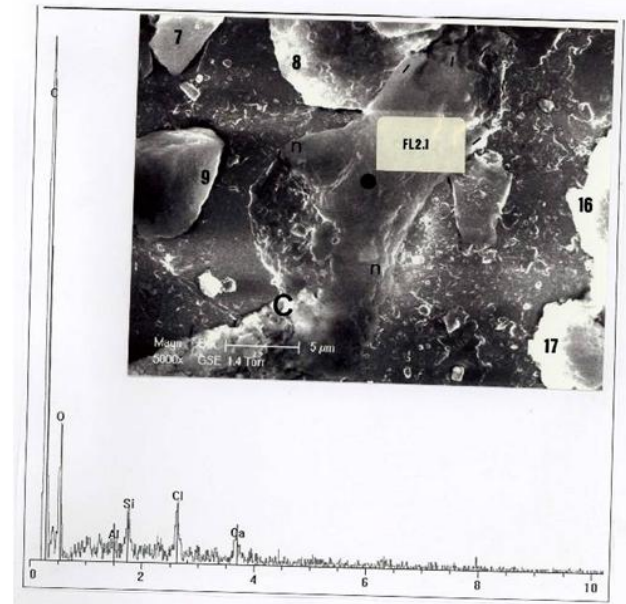
Figure 4. The second (FL2) linen fiber (b10), located in area B. Above, SEM photograph (x5000) of FL2.1 (the upper part of FL2). Below, EDX analysis at the black point
