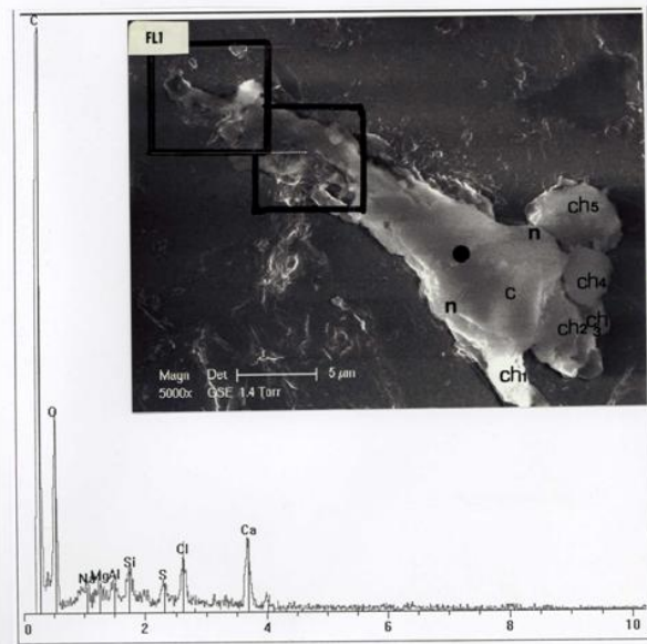
Figure 2. The first (FL1) linen fiber (b11), located in area B of the triangle. Above, SEM photograph (x5000) of FL1 (the two square quadrate parts of the fiber located on its top are magnified in the following figure). Below, EDX analysis (horizontal axis is graduated in keV/V, and heights of the peaks are proportional to quantities of elements in the sample) of FL1 at the black point indicated on the fiber. The two letters n correspond to two borders of the node ; c corresponds to the fiber part composed of calcium carbonate ; ch1-5 are round sub-particles located at the basis of the fiber.
