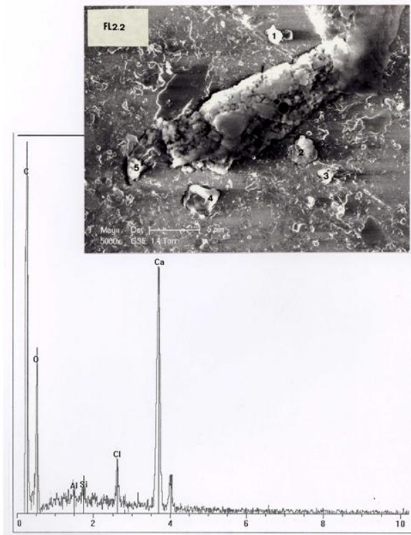
Figure 5. FL2.2 is the lower part of FL2. Above, SEM photography (x5000) of FL2. Below, EDX analysis at the black point indicated. 1,2,3,4 and 5 are little particles of calcite adjacent to FL2.2.
