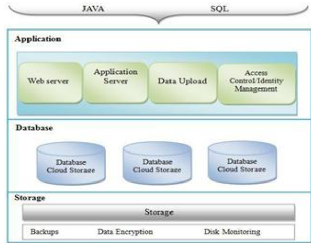
Fig 2. DBMS in Cloud Architecture
