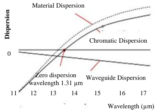
Figure 2 Chromatic Dispersion in a Standard SMF [8].
