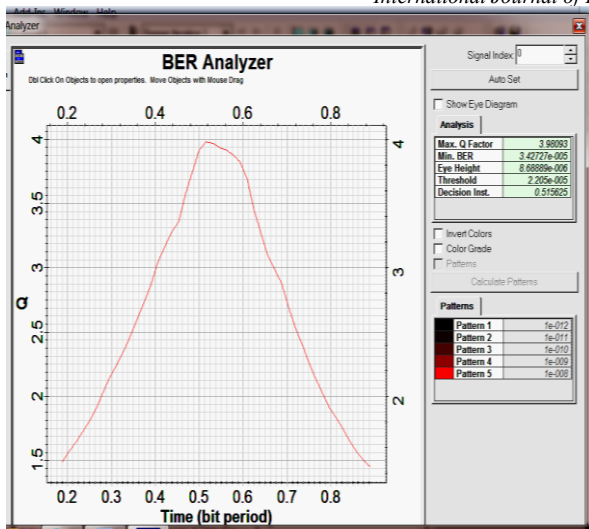
Figure 14. Received Optical Signal of Fiber length 130 km after using FBG
