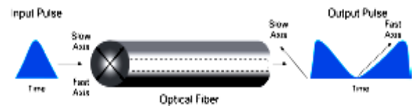
Figure3. Pulse Splitting Due to PMD in a Single-Mode Fiber
