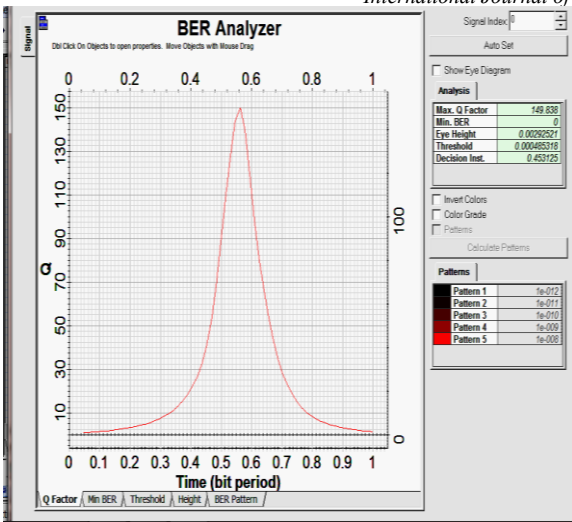
Figure8. Initial Optical Signal
