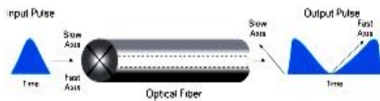
Figure3. Pulse Splitting Due to PMD in a Single-Mode Fiber
