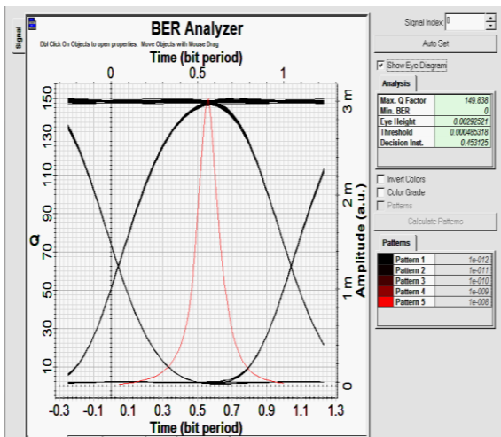
Figure 9. Initial Optical Signal Represented by the Eye Diagram
