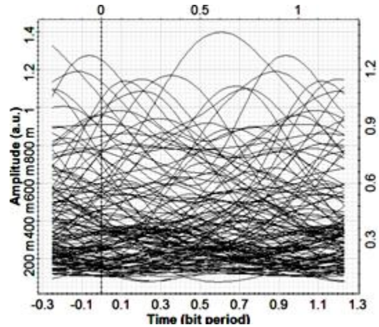
Figure 8 Eye diagram analyzer for the received signals ta distance grater than 60 km.
