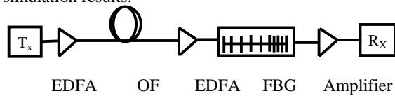
Figure6. Fiber-optic Transmission link System Block Diagram
