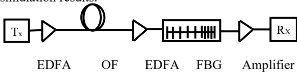
Figure6. Fiber-optic Transmission link System Block Diagram
