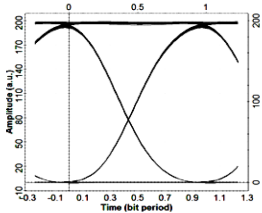
Figure 7 Eye diagram analyzer shows that the digital '1' and '0' levels of the received bids are easy to distinguish.
