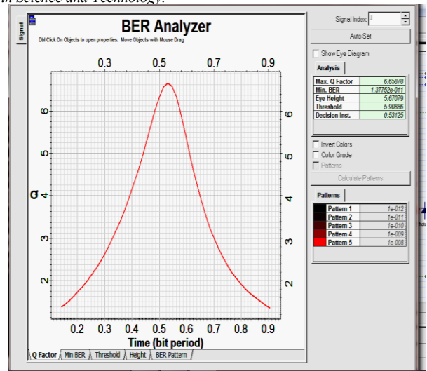
Figure 12. Output Optical Signal output at 100 km when FBG is used.
