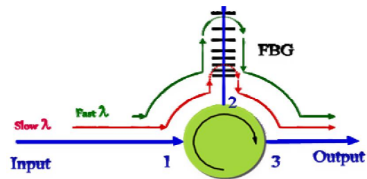
Figure5. Optical Circular Scheme [13].
