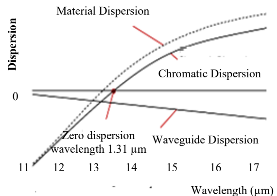
Figure 2 Chromatic Dispersion in a Standard SMF [8].
