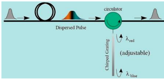
Figure 6 Chromatic Dispersion Compensation using FBG and Circular [11-13].
