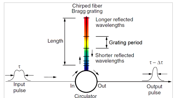
Figure 4 Layout of a Fiber Bragg Grating Based Dispersion Compensation Module [13].
