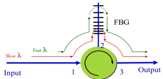
Figure5. Optical Circular Scheme [13].
