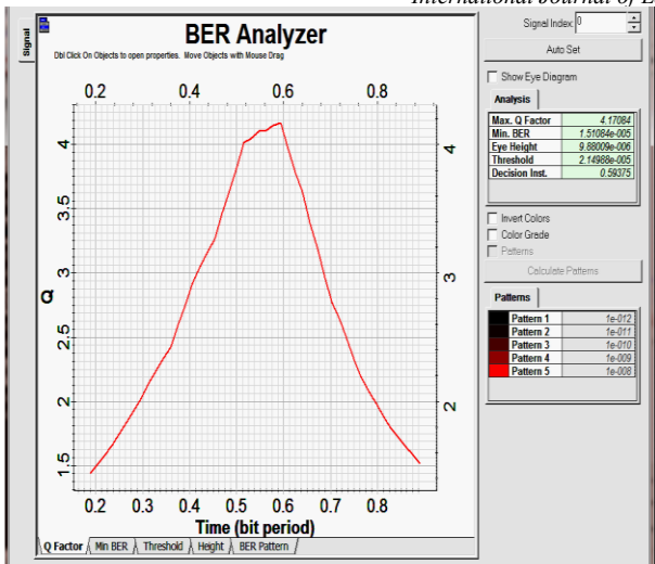
Figure10. Received Optical Signal at 100km
