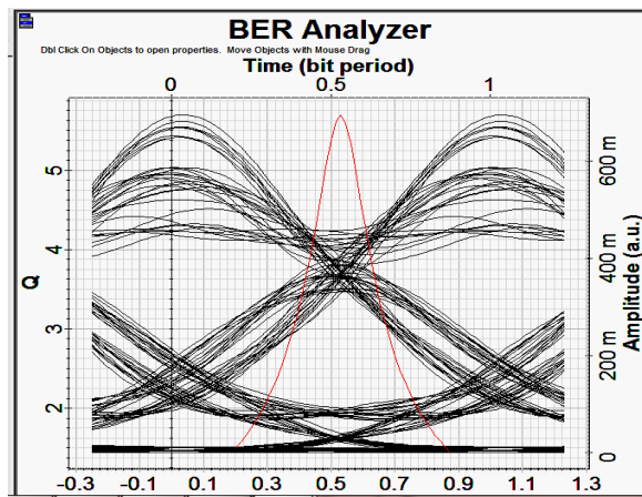
Figure11. Optical Output Signal eye diagram at distance 100km after applying the amplifier
