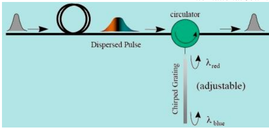
Figure 6 Chromatic Dispersion Compensation using FBD and Circular [11-13].
