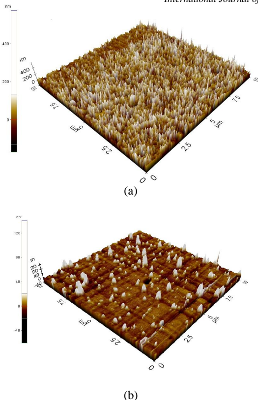
Figure 5 Two typical 3-dimensional AFM images of (a) as-deposited a-C film and (b) boron doped a-C film
