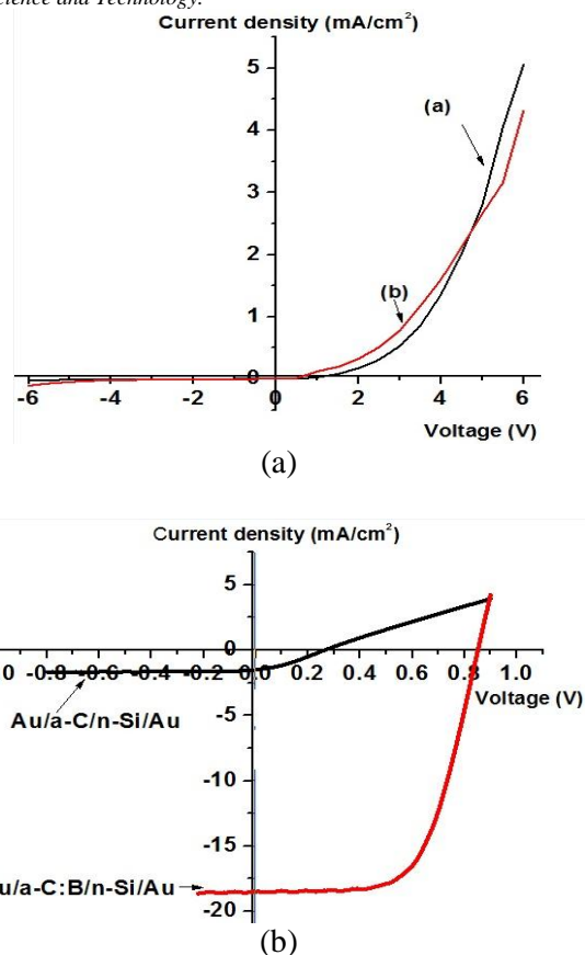
Figure 6 The Au/a-C/n-Si/Au and Au/a-C:B/n-Si/Au solar cells under dark and illumination at 0 V and -20 V
