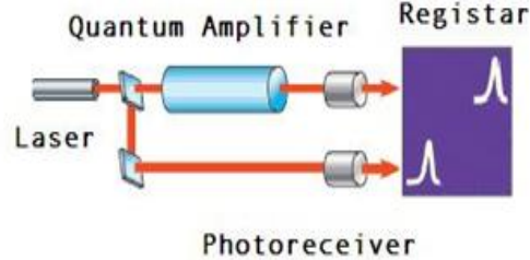
Figure 5. Experiments of L.Wang - superluminal light propagation.
