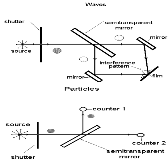
Figure 1. Experiments with individual photons on semitransparent mirror.
