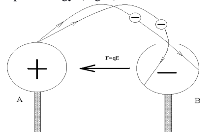
Figure 7. Work for transferring the charge depends on the mode of transferring and on the path.
