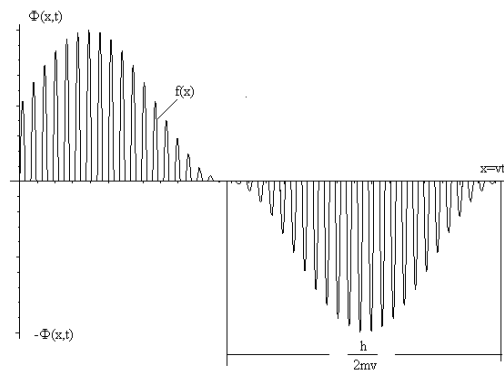
Figure 2. Behaviour of wave packet in linear dispersion medium (i.e., rather like a series of stroboscopic photographs).
